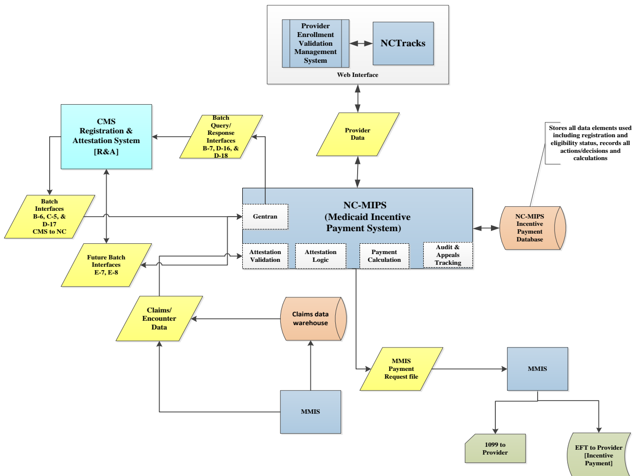
Figure 16 - NC-MIPS Integration
